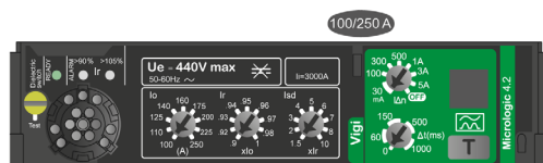
Micrologic 4 trip
