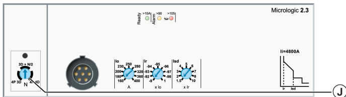
Micrologic 2.3 4P version
