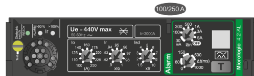
Micrologic 4 alarm
