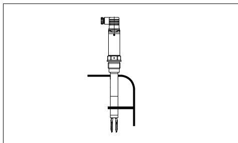
Fig. 17: Lateral support of LFV 230
