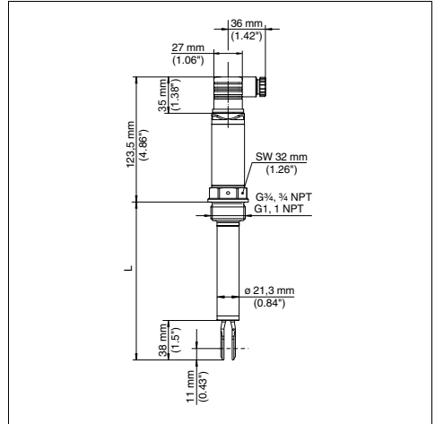
Fig. 24: LFBV 230, high temperature version with valve plug acc. to ISO 4400 L = Sensor length, see chapter "Technical data"
