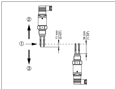
Fig. 13: Vertical mounting
