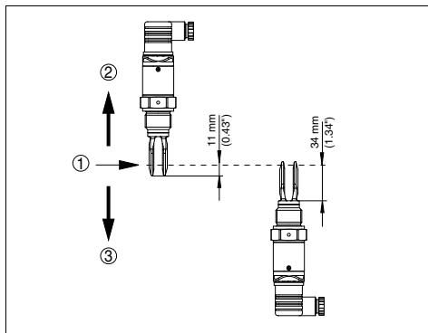
Fig. 25: Montage vertical
