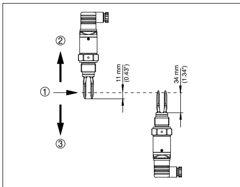
Fig. 13: Vertical mounting
