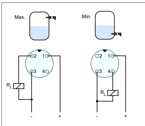
Fig. 20: Wiring plan (housing), transistor output with M12 x 1 plug connection
