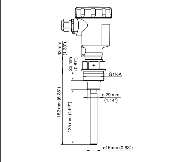
Fig. 33: LBV 311 - threaded version G1½ A (DIN ISO 228/1)
