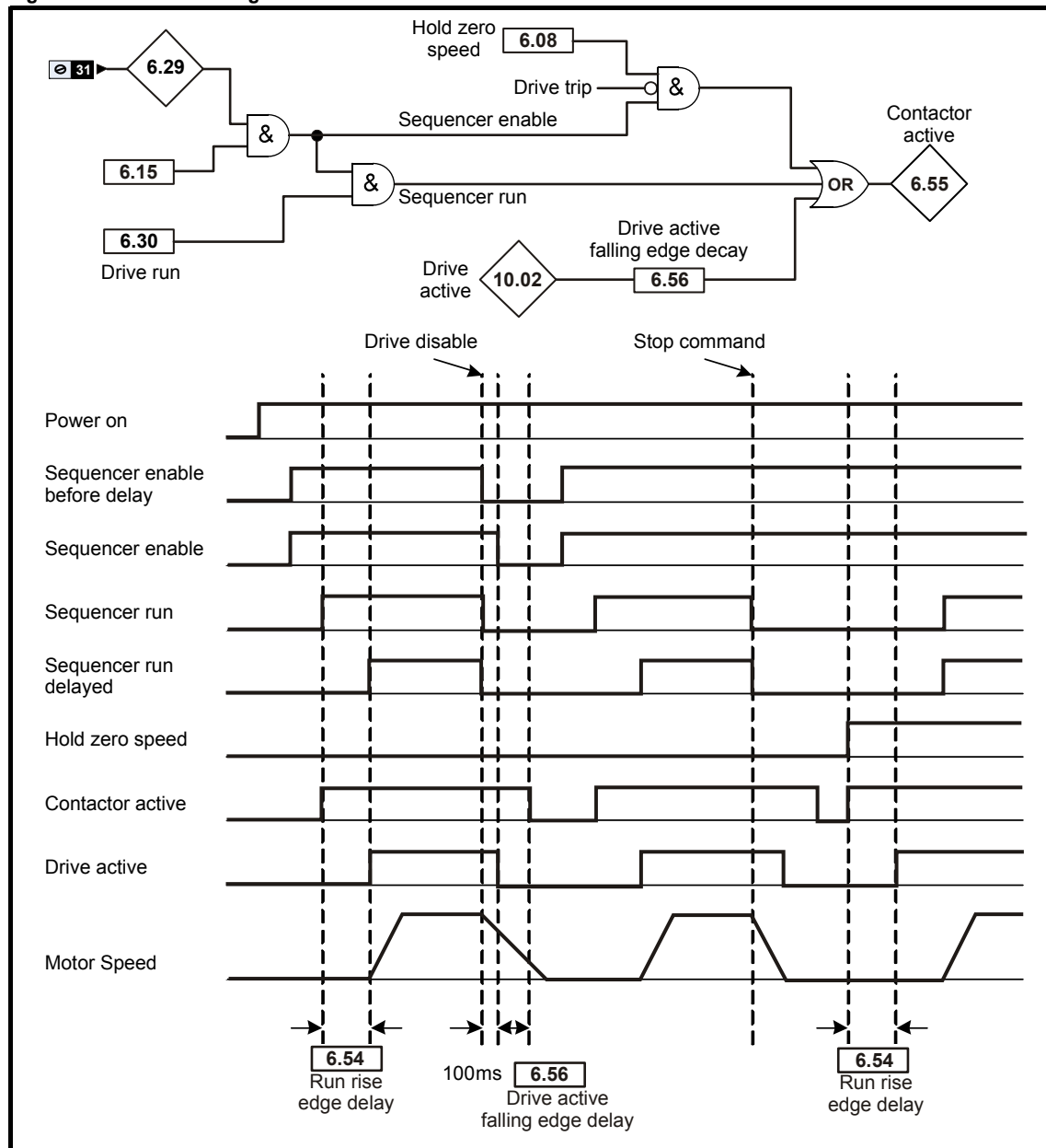
Figure 5-22 Contactor logic
