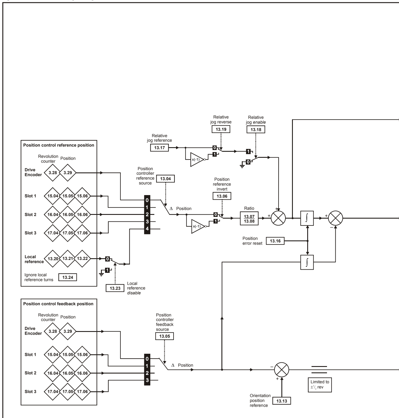
Figure 5-33 Menu 13 logic diagram
