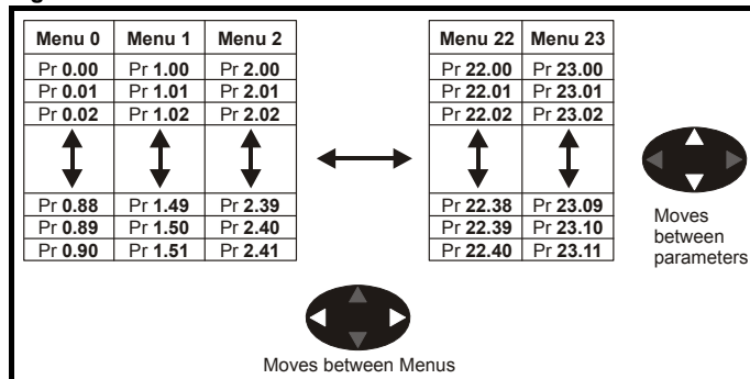
Figure 1-2 Menu structure
