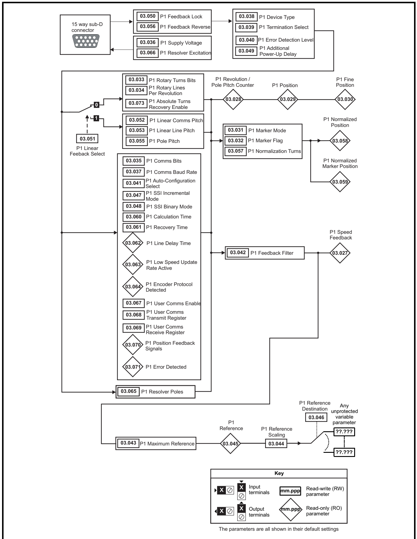
Figure 12-5 P1 Interface
