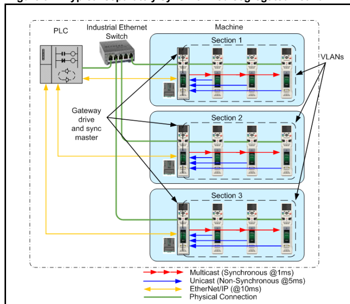
Figure 9-4 Typical separately synchronized segregated network
