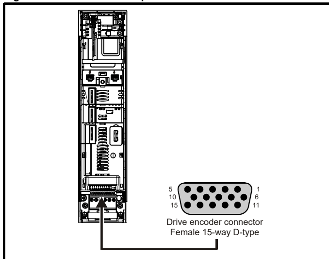
Figure 4-9 Location of the position feedback
