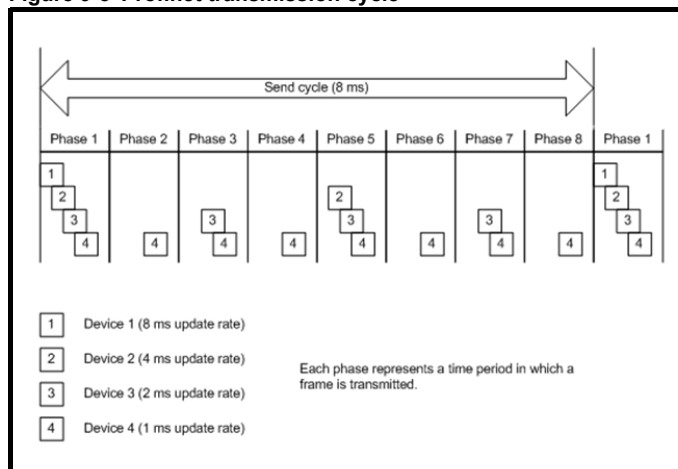
Figure 9-5 Profinet transmission cycle
