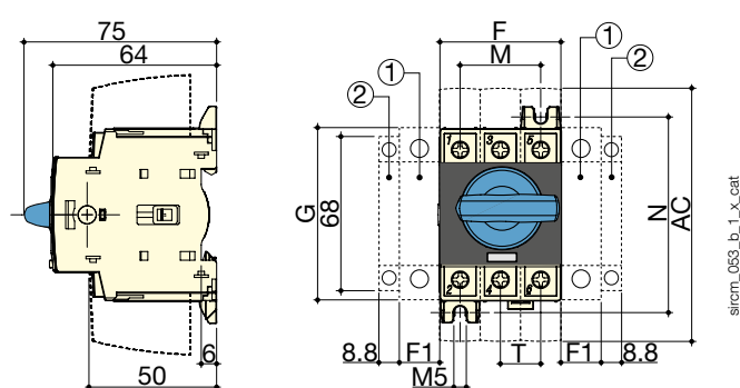
Direct operation with handle
