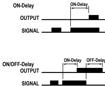
Figure 2. Timing Diagrams and Adjustment Locations
