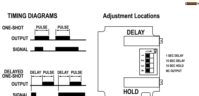
Figure 3. Timing Diagrams and Adjustment Locations
