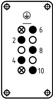
contact arrangement (view from termination side)
