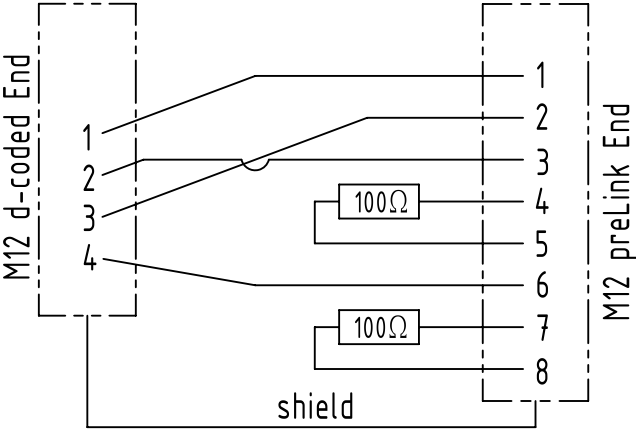
circuit diagram
