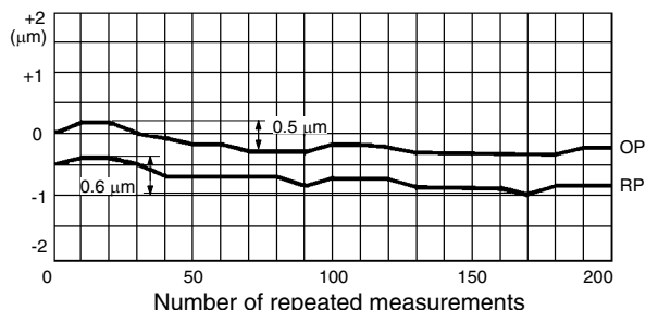
M8 Type (Contact/Solid-state Output) With Repeat Accuracy of 1 \mu\text{m} max. D5A-3□□□ Series
