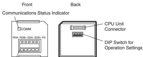
RS-422A/485 Connector
