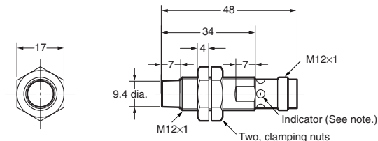
E2A-M12KN08-M1-□□/E2A-S12KN08-M1-□
