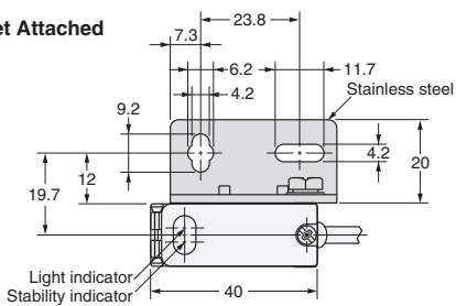
Mounting Holes
