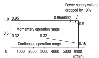
R88M-K75030H/T (750 W)
