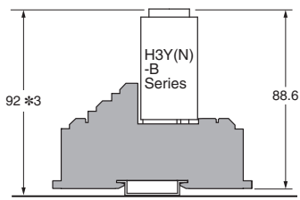
PYF-08-PU-L (PYF-14-PU-L)
