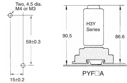
Mounting Holes
