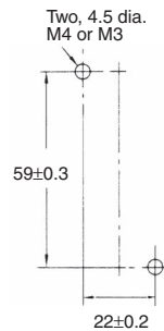
Mounting Holes
