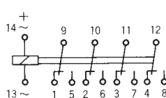
(DIN notation)
