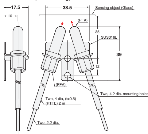
55-H E32-L11FS 2M (Free Cutting)
