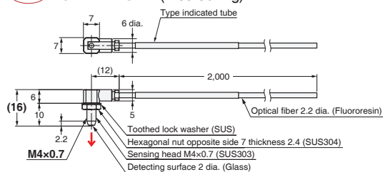
39-A2 E32-T11NFS 2M (Free Cutting)
