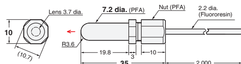
39-C E32-T11F 2M (Free Cutting)
