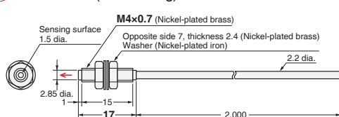
(45-B) E32-T51 2M (Free Cutting)
