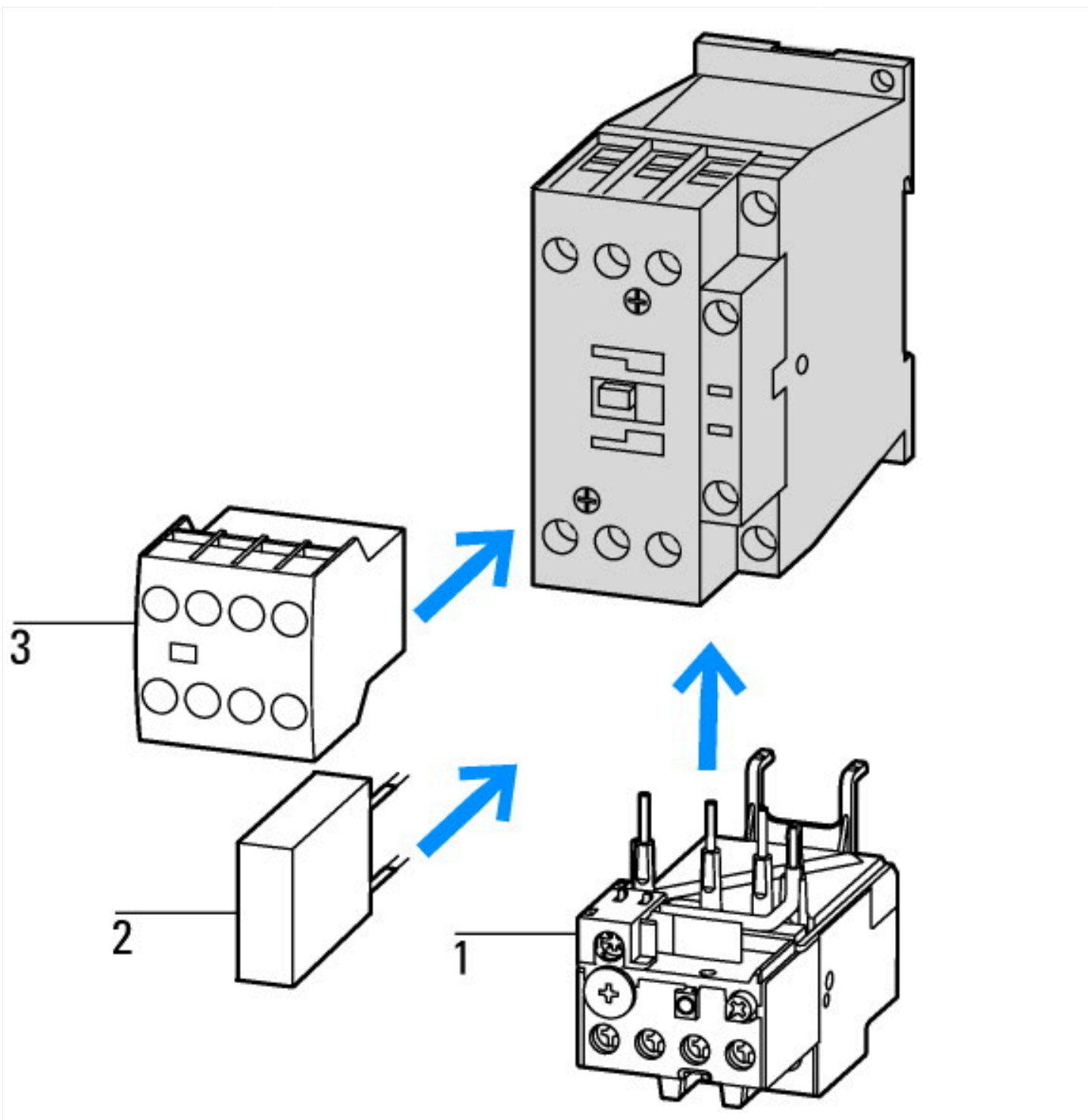
1: Overload relay
