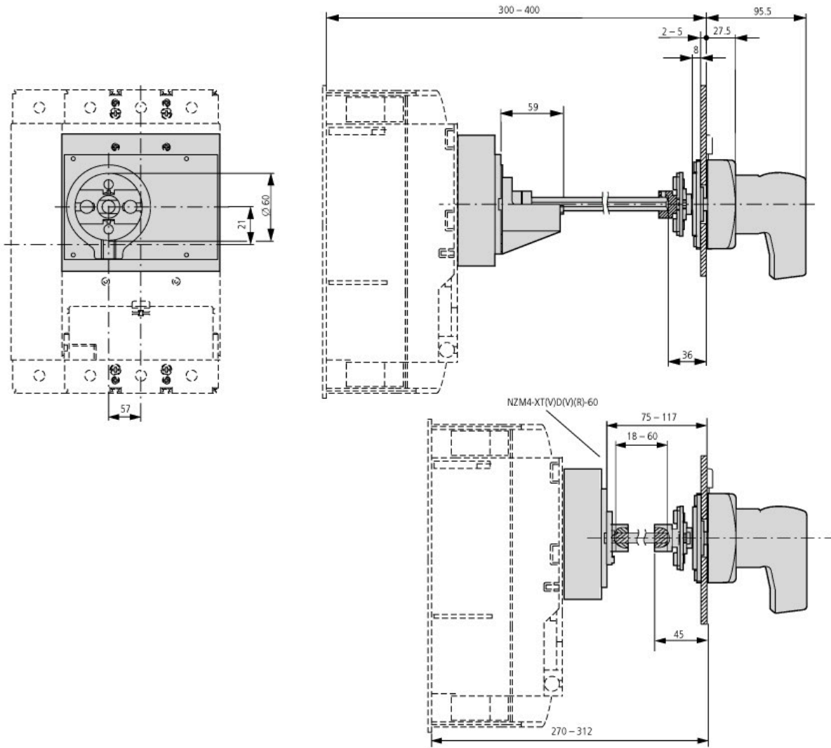
in connection with NZM4-XT(V)D(V)(R) door coupling rotary handle
