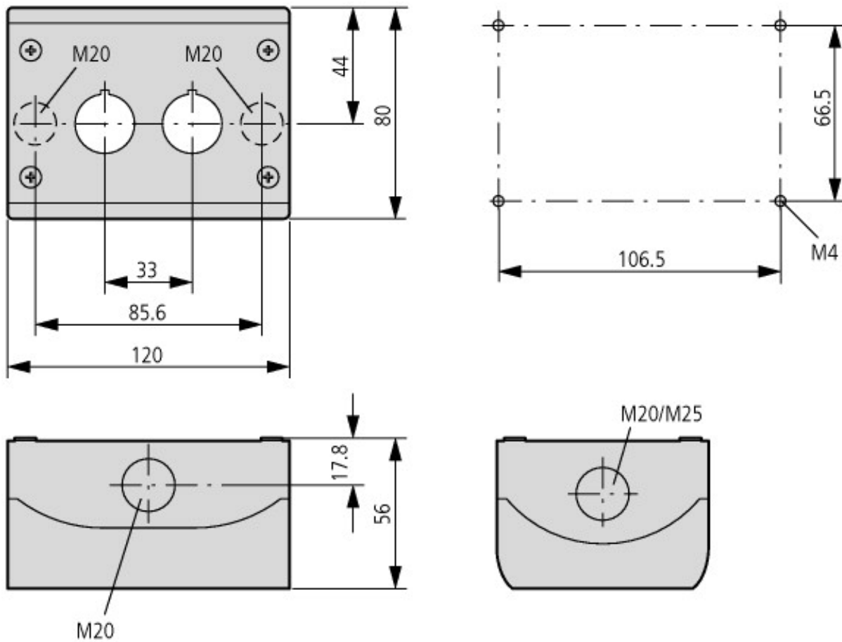
Premoulded cable entry: bottom 2 x M20, top: 1 x M20, side: 2 x M20/M25 (per side 1 x)
