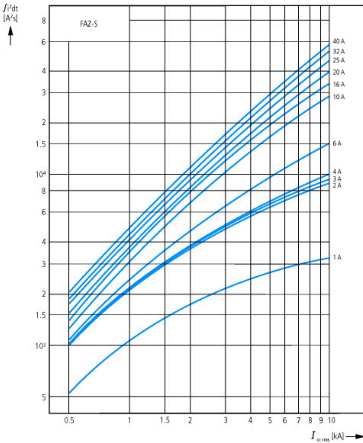
Let-through current \hat{i}_p According to IEC/EN 60898
