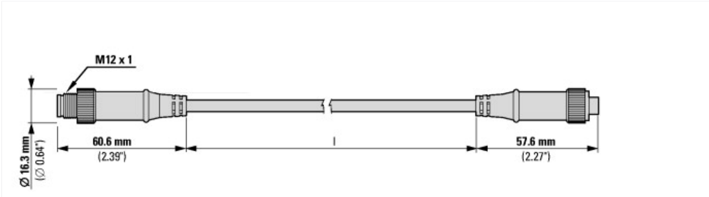
M12 SWD round cable, 5 pole
