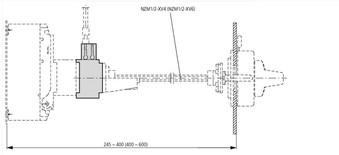
NZM1-XMV + NZM1-XTVD(V)(R)
