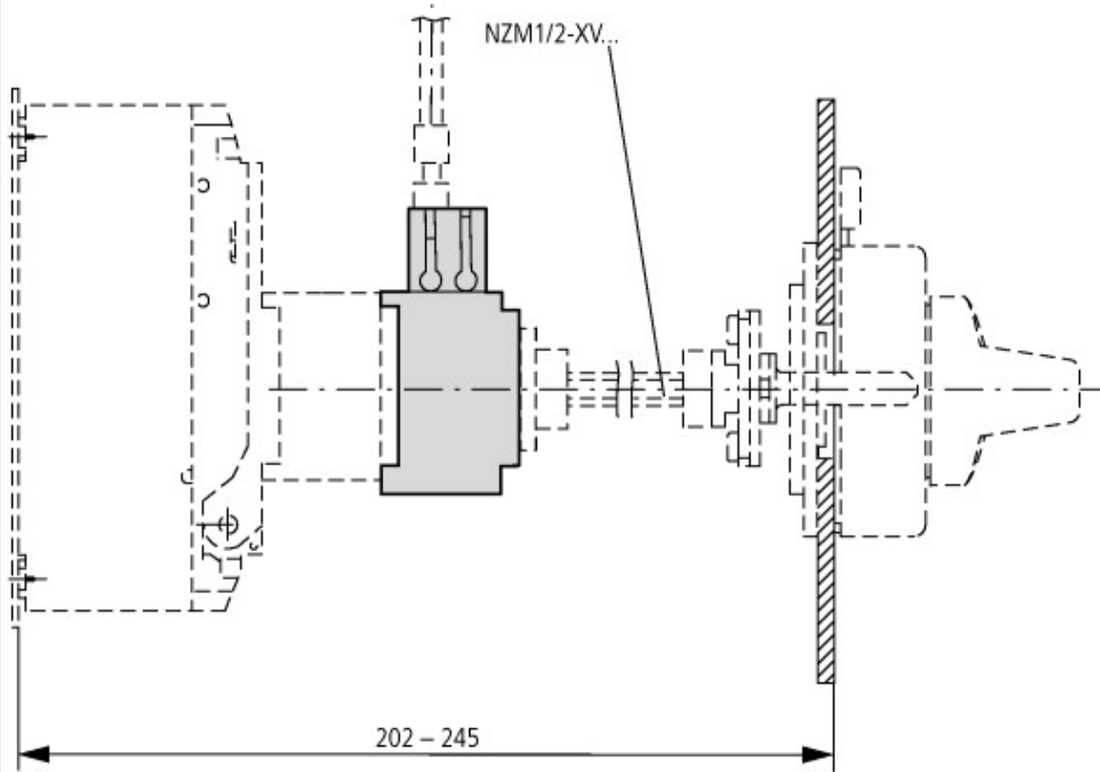
NZM1-XMV + NZM1-XTVD(V)(R)-60
