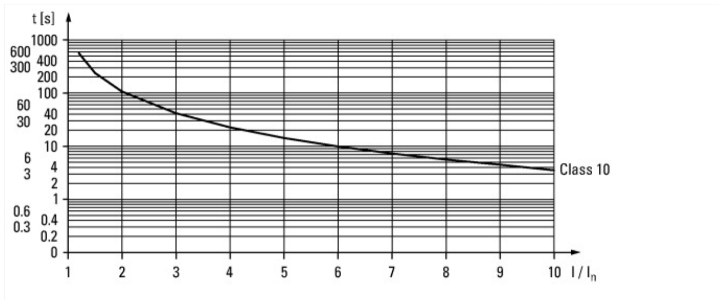
Tripping characteristics CLASS 10 set motor current \leq 4 A
