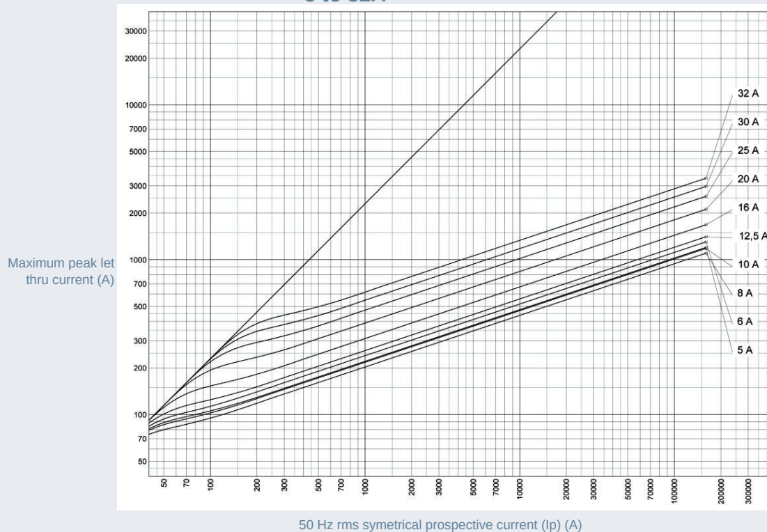
Peak let thru characteristics 5 to 32A
