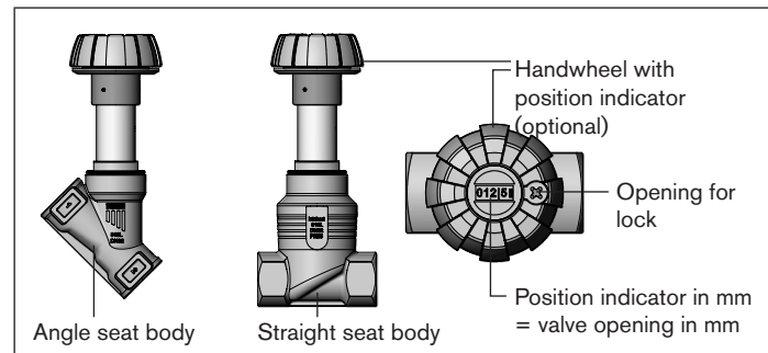
Fig. 2: Valve types
