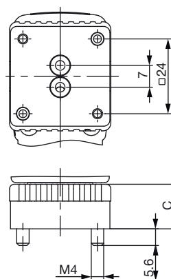
Sub-base version (SFB) underside view
