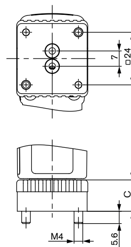
Flange version (SFB)
