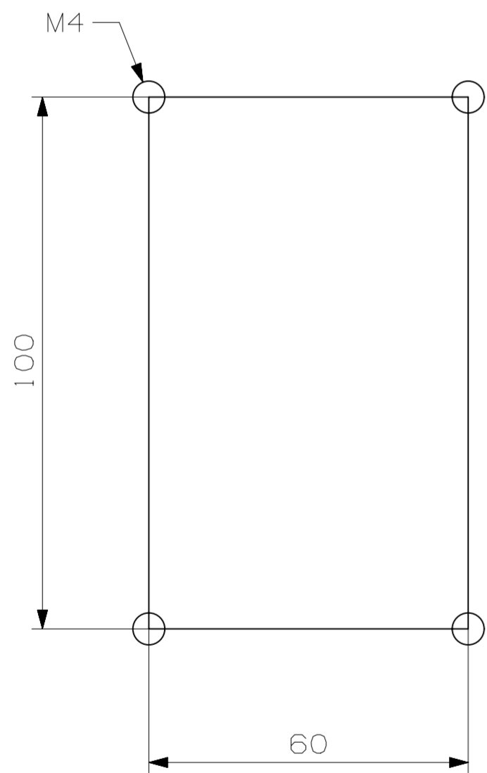
Drilling plan
