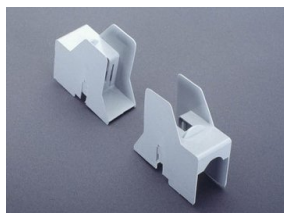
03791 shock protection in two parts for NH fuse-base size 00 particular article
