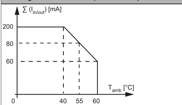
BWU3577, BWU3695 Derating total current of inputs and outputs
