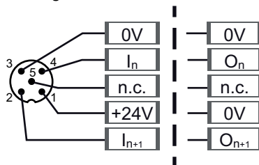
Y-wiring
