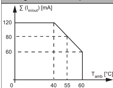
BWU3326, BW3500, BWU3639 Derating total current of inputs and outputs
