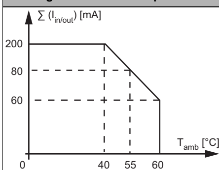
BWU3606 Derating total current of inputs and outputs
