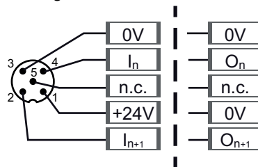
Y-wiring
