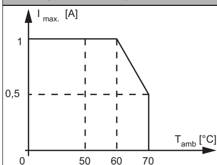
BW3250 Derating power supply of attached sensors
