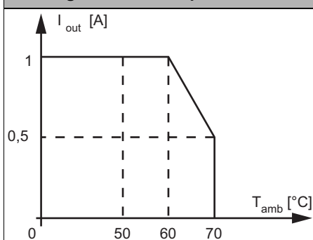
BW3250 Derating current of output
