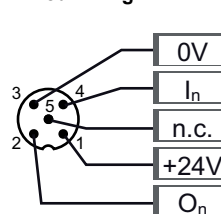
Mixed-wiring
