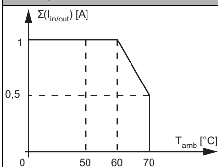
BWU3497, BWU3602, BWU3628 Derating total current of inputs and outputs
