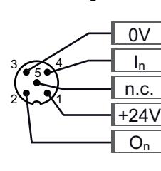
Mixed-wiring
