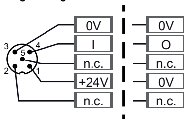
Single-wiring
