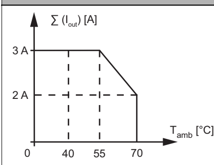
BWU2594, BWU2713, Derating total current of outputs
