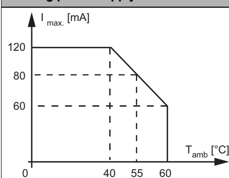
BWU3317, BW3507, BWU3555 Derating power supply of attached sensors
