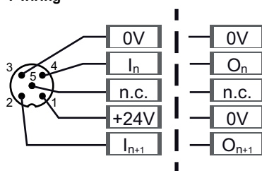
Y-wiring
