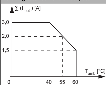
BWU3317, BW3507, BWU3555, BWU3785 Derating total current of outputs
