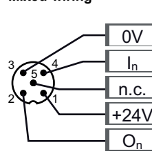
Mixed-wiring
