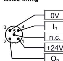
Mixed-wiring
