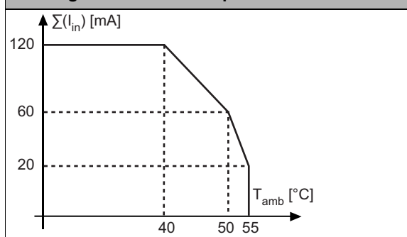
(4) BWU3747 Derating total current of inputs
