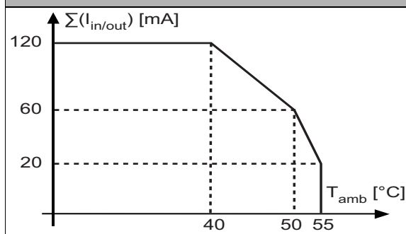
(2) BWU2783, BWU3272 Derating total current of inputs + outputs
