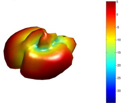
Freq = 2.41GHz Az= 45 EL= 45
