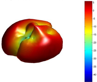
Freq = 2.1GHz Az= 45 EL= 45
