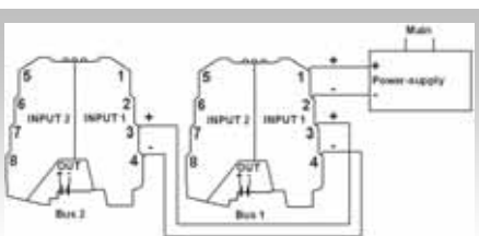
Example of connection to more than one bus
