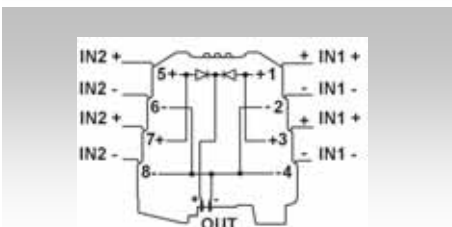
Internal wiring
