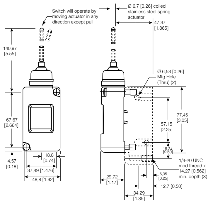
Figure 23. 208LS152 Dimensions
