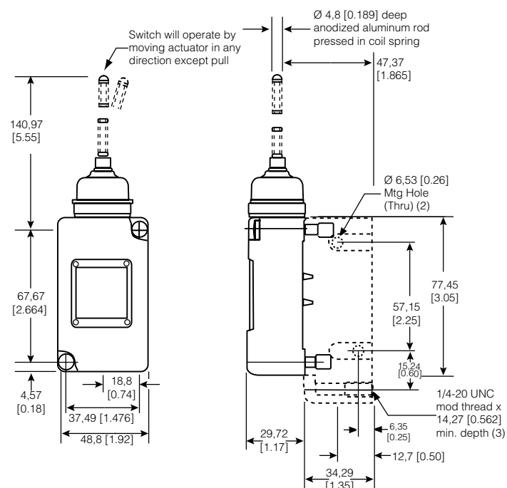
Figure 21. 208LS3 Dimensions
