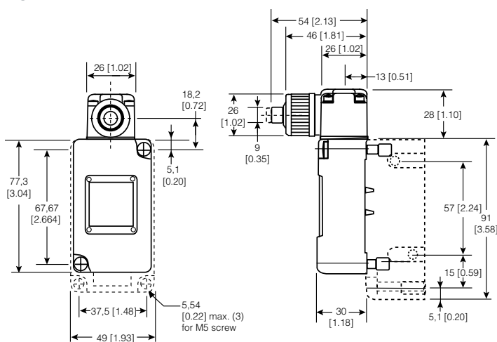
Figure 37. 204LS1-4 Dimensions
