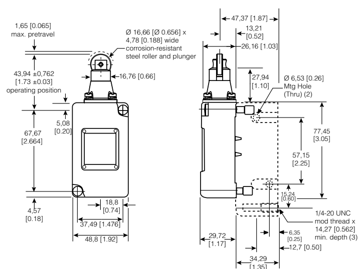
Figure 19. 206LS1 Dimensions
