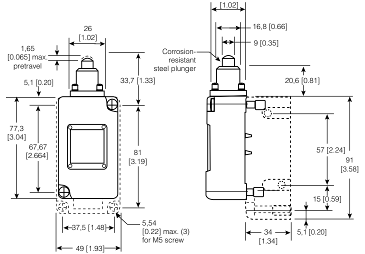
Figure 39. 208LS1-4 Dimensions
