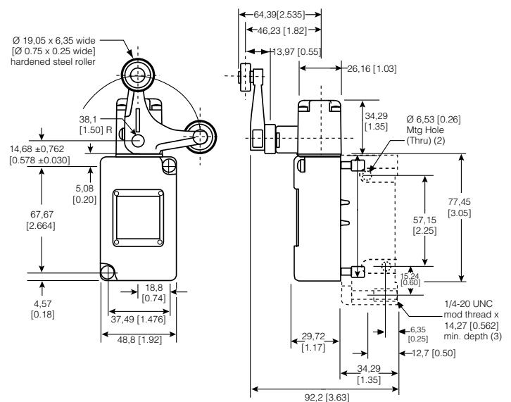
Figure 19. 206LS1 Dimensions
