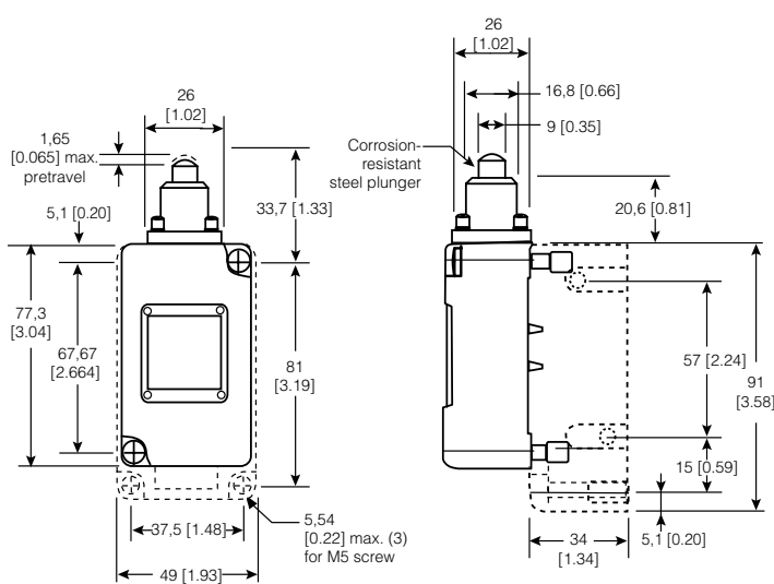
Figure 37. 204LS1-4 Dimensions
