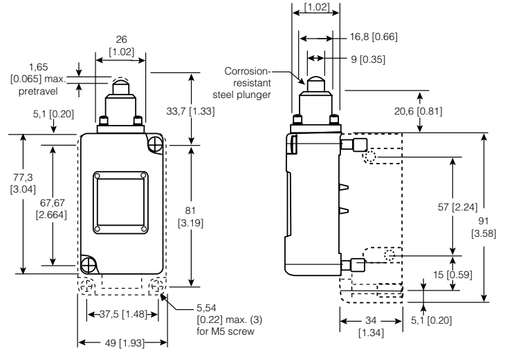
Figure 39. 208LS1-4 Dimensions
