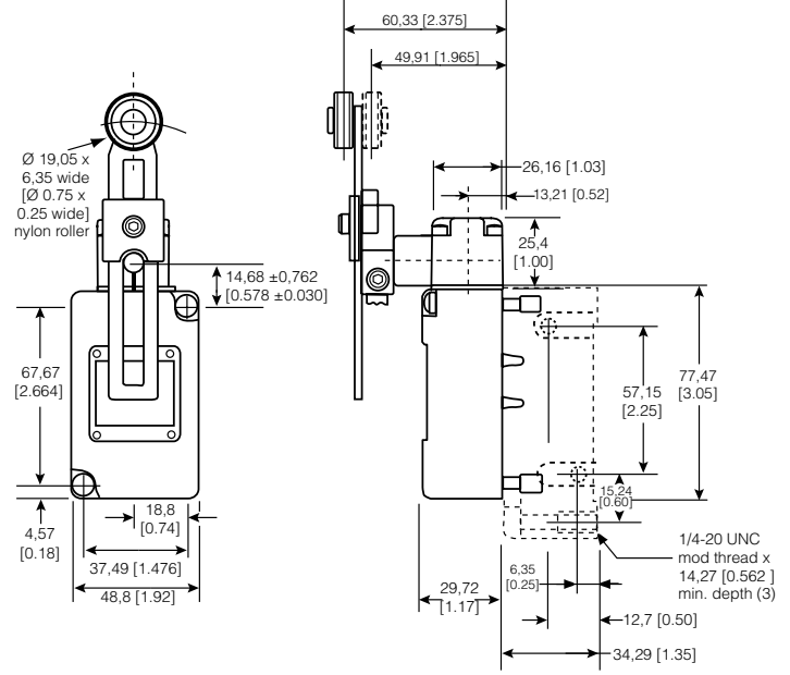
Figure 13. 201LS3 Dimensions
