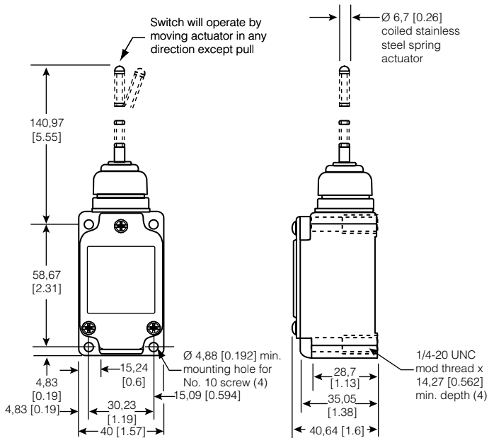
Figure 11. 8LS152 Dimensions
