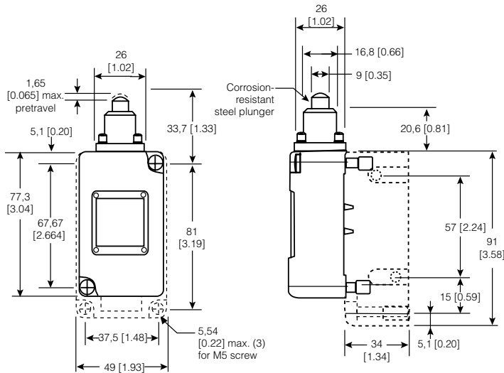
Figure 37. 204LS1-4 Dimensions
