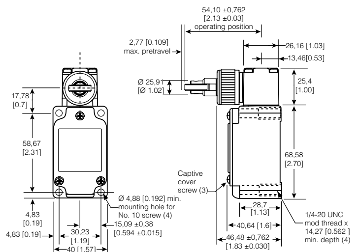
Figure 6. 4LS1 Dimensions
