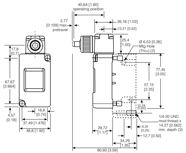
Figure 18. 205LS1 Dimensions
