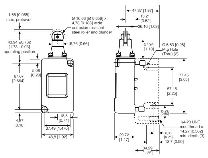
Figure 19. 206LS1 Dimensions
