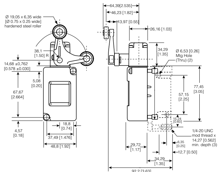
Figure 19. 206LS1 Dimensions
