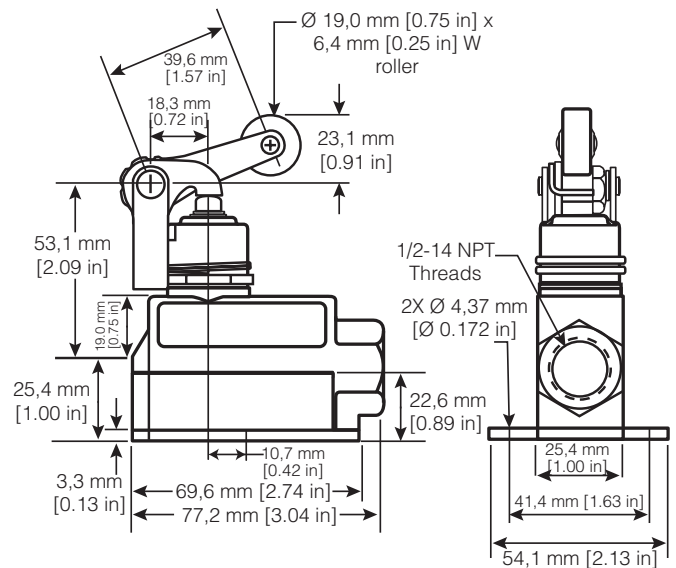
Figure 28. Roller lever adjustable, flange mount with boot seal
